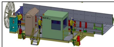
Figure 2: New Design of Hot Car
